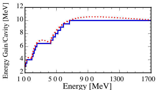
Figure 1: Maximum (upper line) and actual (lower line) energy gain along the accelerator as a function of the beam energy, assuming a peak surface field of 15 MV/m and synchronous phase \phi_s = -30^\circ .
