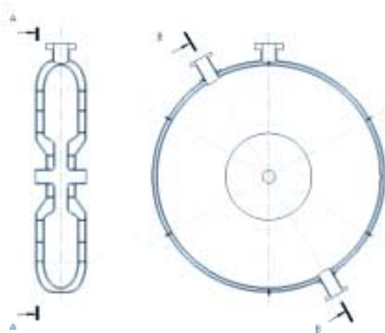
Fig.1 Mechanical design of the reentrant cavity.
