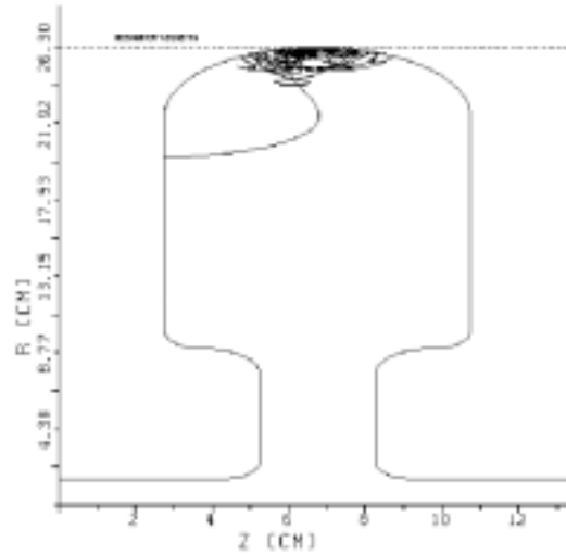
Fig.2. Example of the multipacting simulation program output (the horizontal axis is stretched in the picture). The circular contour, as well as the rectangular one, was causing high field multipacting levels.
