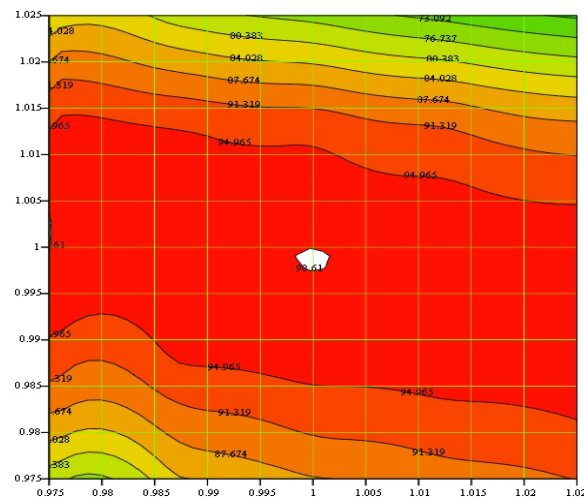
Figure 9: Beam transmission through LEBT and RFQ as a function of the two LEBT solenoid currents, normalized at the nominal value.
