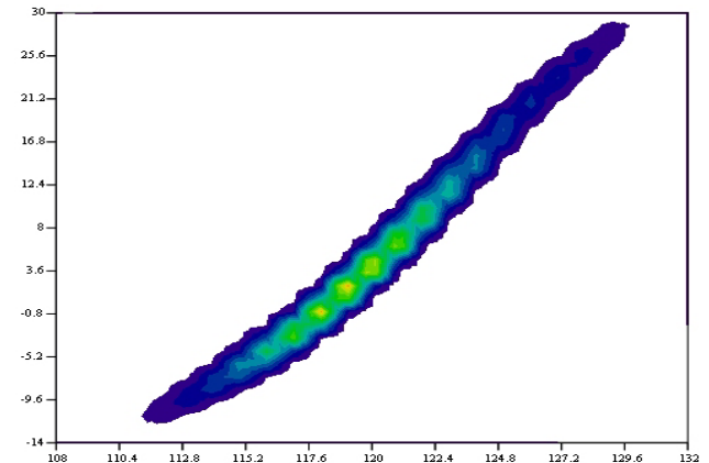
Figure 5: Proton beam emittance measurement with neutralization. V_{ext}=80 KV, V_{puller}=35 KV, I_{magnet}=280 A, P_{source+Ar}=2.5 E-5 mbar, P_{line+Ar}=3.6 E-5 mbar.
