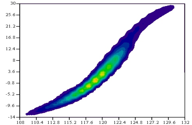
Figure 4: Proton beam emittance measurement without neutralization. V_{ext}=80 KV, V_{puller}=35 KV, I_{magnet}=280 A, P_{source}=1.3 E-5 mbar, P_{line}=6.9 E-6 mbar.
