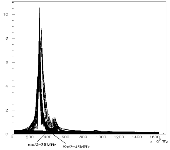
Fig. 2:Overlapping of FFT of some particle beam trajectories with initial x positions taken from 0.07 to 0.18 cm. The beam radius, after the Debye length tail is formed, is about 0.2.
